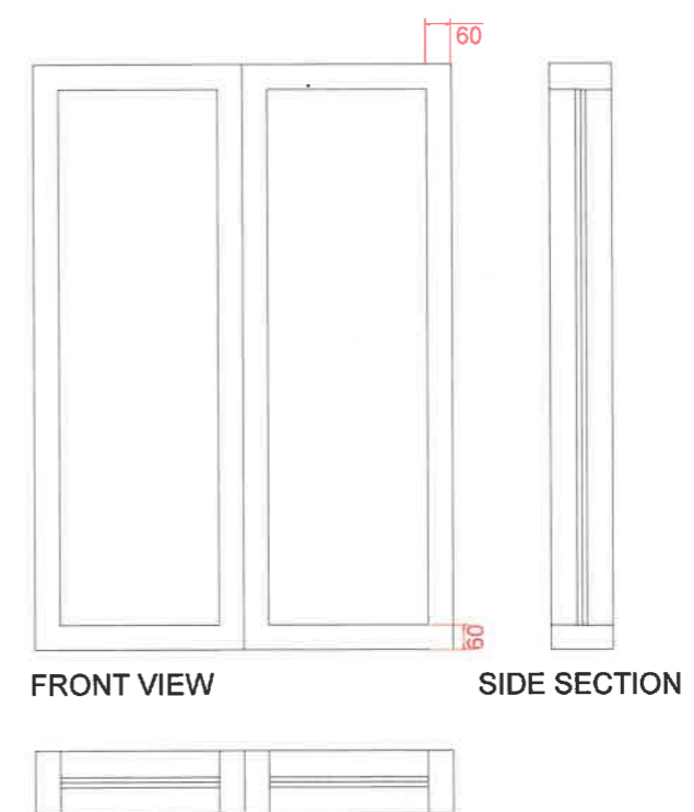
CASEMENT WINDOW TYPICAL DETAIL - SCALE 1:10
