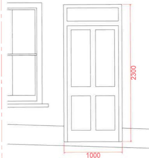
ELEVATION B - SCALE 1:20 MATERIAL : PAINTED SOFTWOOD
