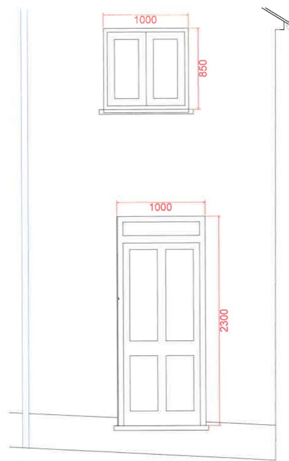
ELEVATION C - SCALE 1:20 MATERIAL : PAINTED SOFTWOOD
