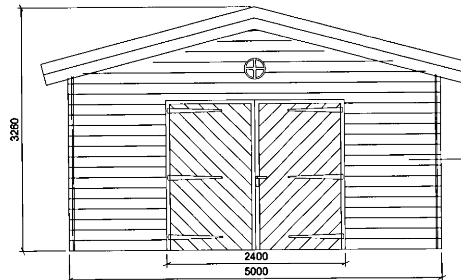
FRONT ELEVATION
