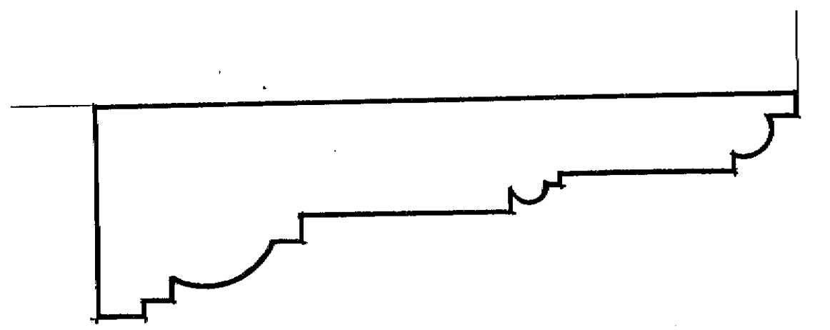
17 ARCHITRAVE TO COMMUNICATING DOOR
