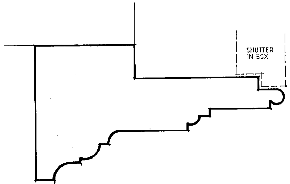
22 ARCHITRAVE TO WINDOWS INTERNALLY
