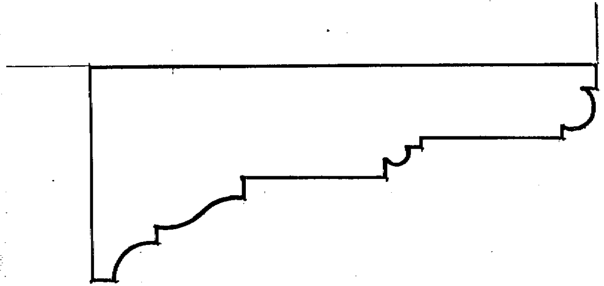
21 ARCHITRAVE TO ENTRANCE DOOR AND OTHER DOOR IN SAME WALL
