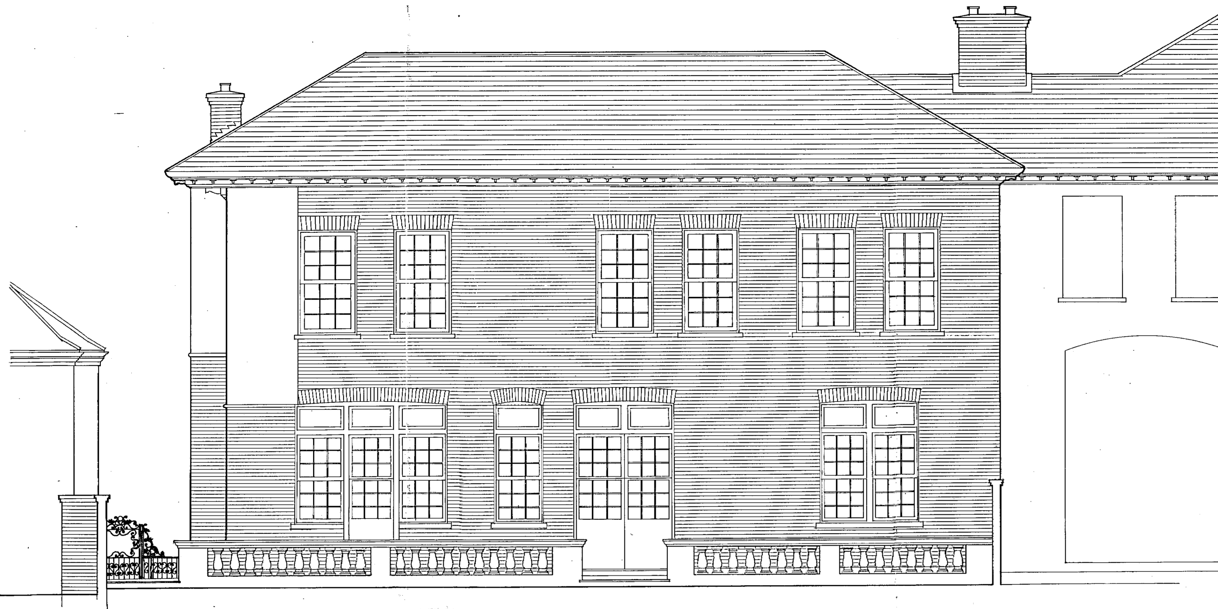
SOUTH FACING ELEVATION
