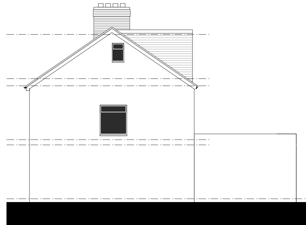
side elevation from 23 manor road
