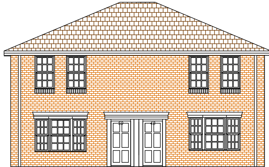
Front Elevation - No.46-52 Rooks Hill
