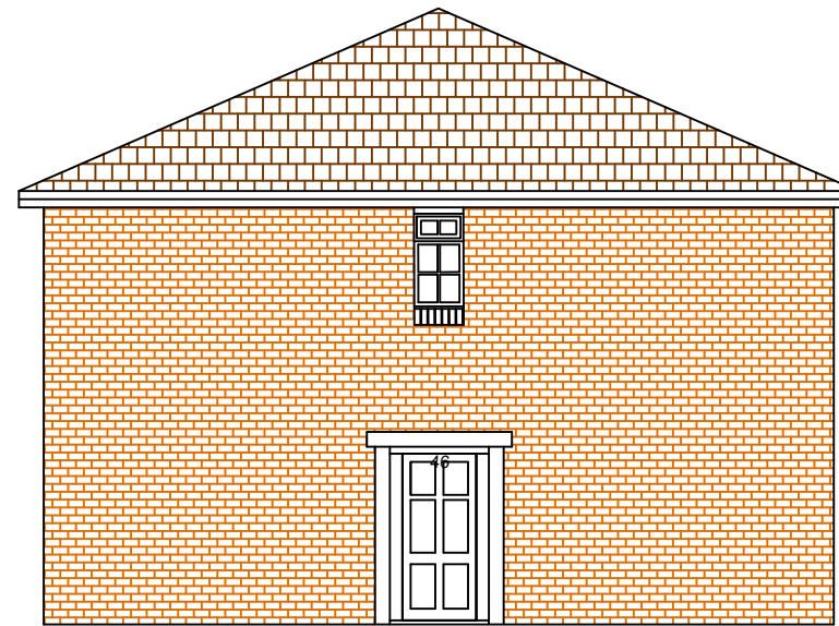
Flank Elevation - No.46-52 Rooks Hill
