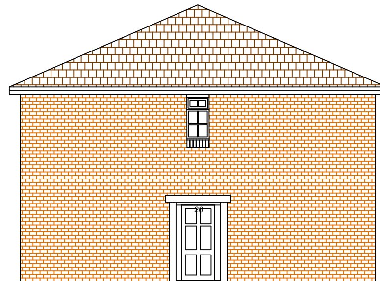
Flank Elevation - No.26-32 Rooks Hill
