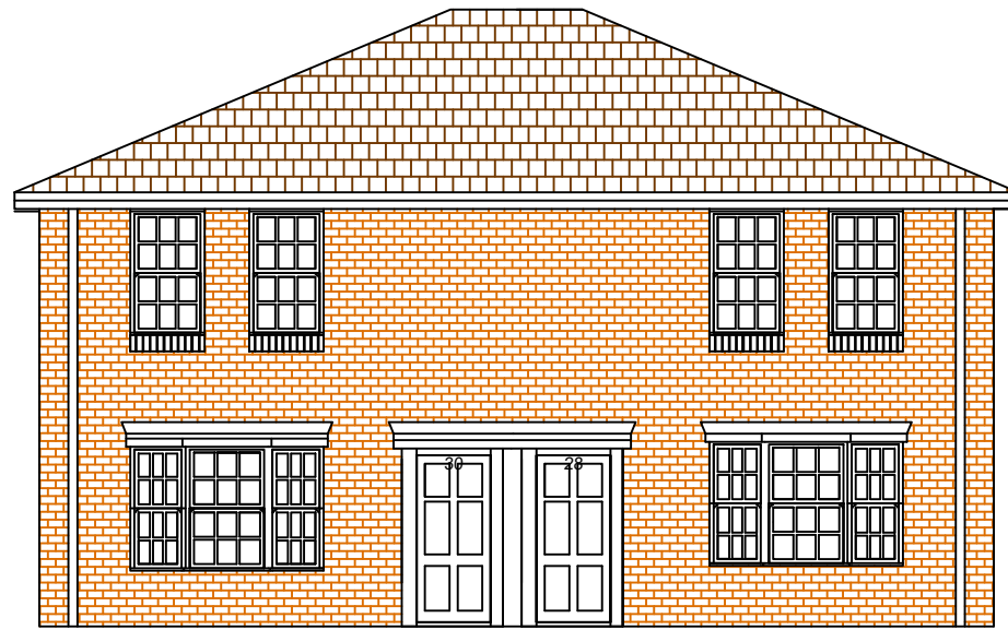
Front Elevation - No.26-32 Rooks Hill
