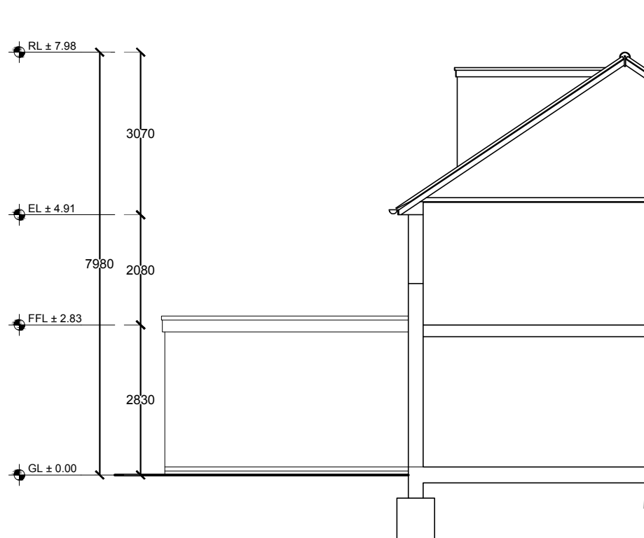
Proposed Side Elevation (Section A-A)
