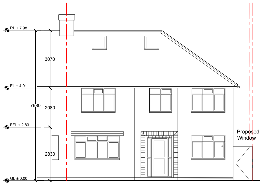
Proposed Front Elevation (North)
