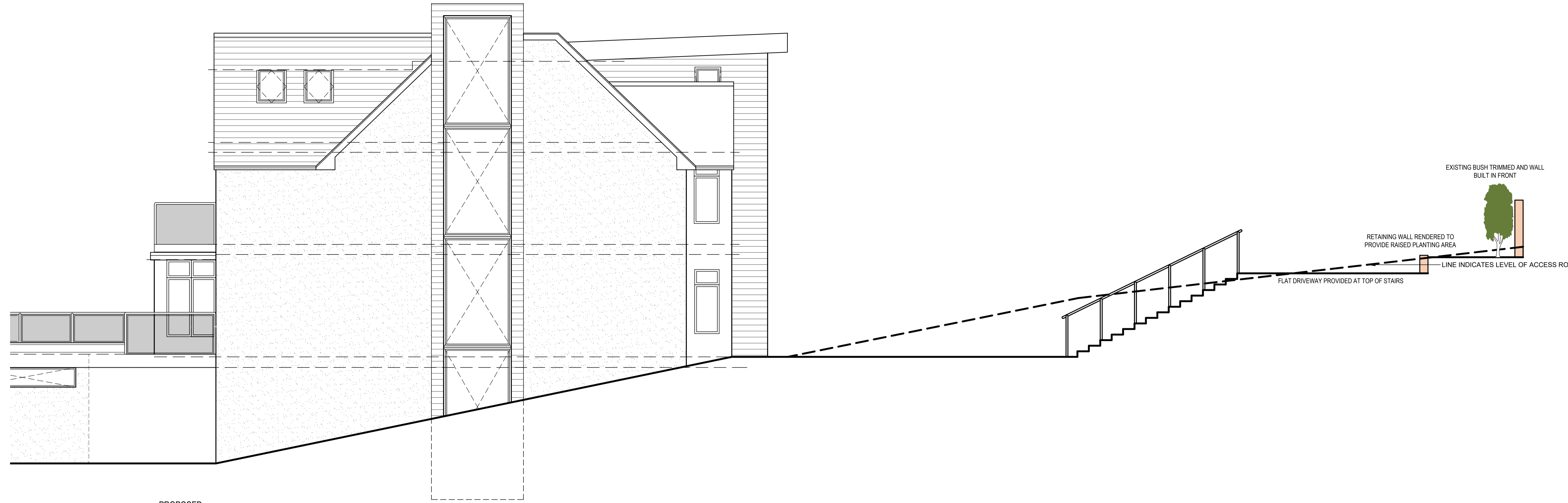
PROPOSED SECTION A-A (scale 1:50)
