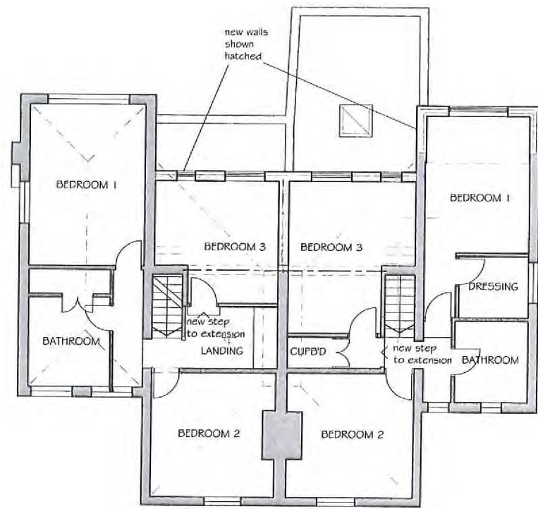
6 4 FIRST FLOOR
