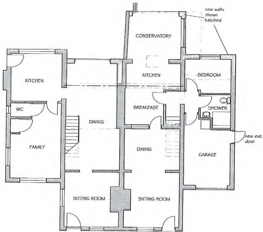
6 4 GROUND FLOOR
