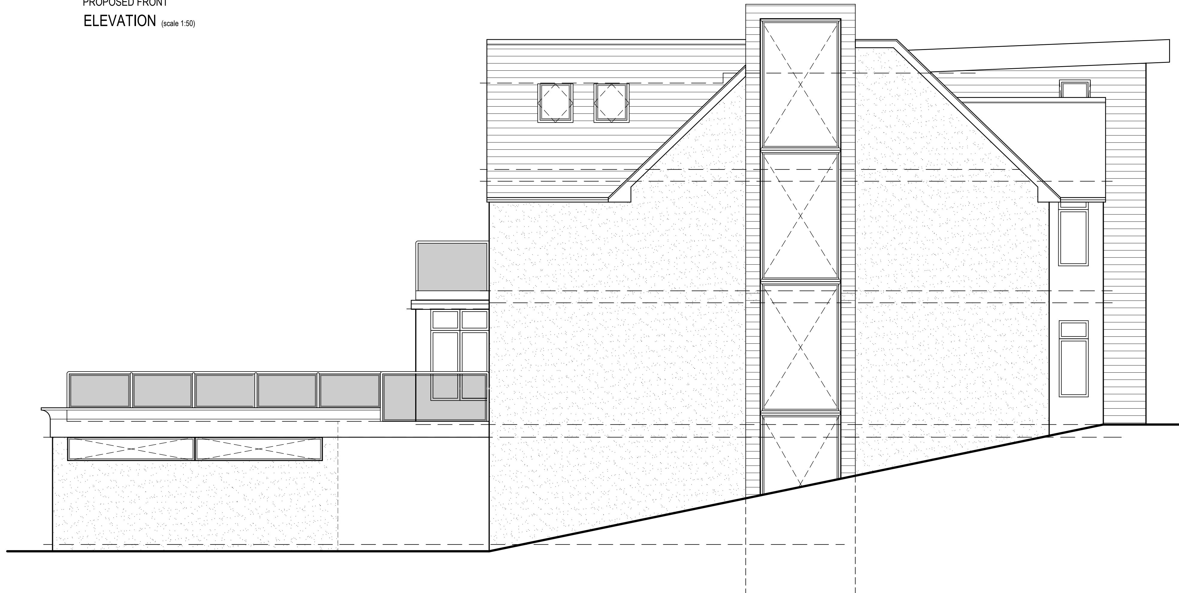
PROPOSED SIDE (1) ELEVATION (scale 1:50)
