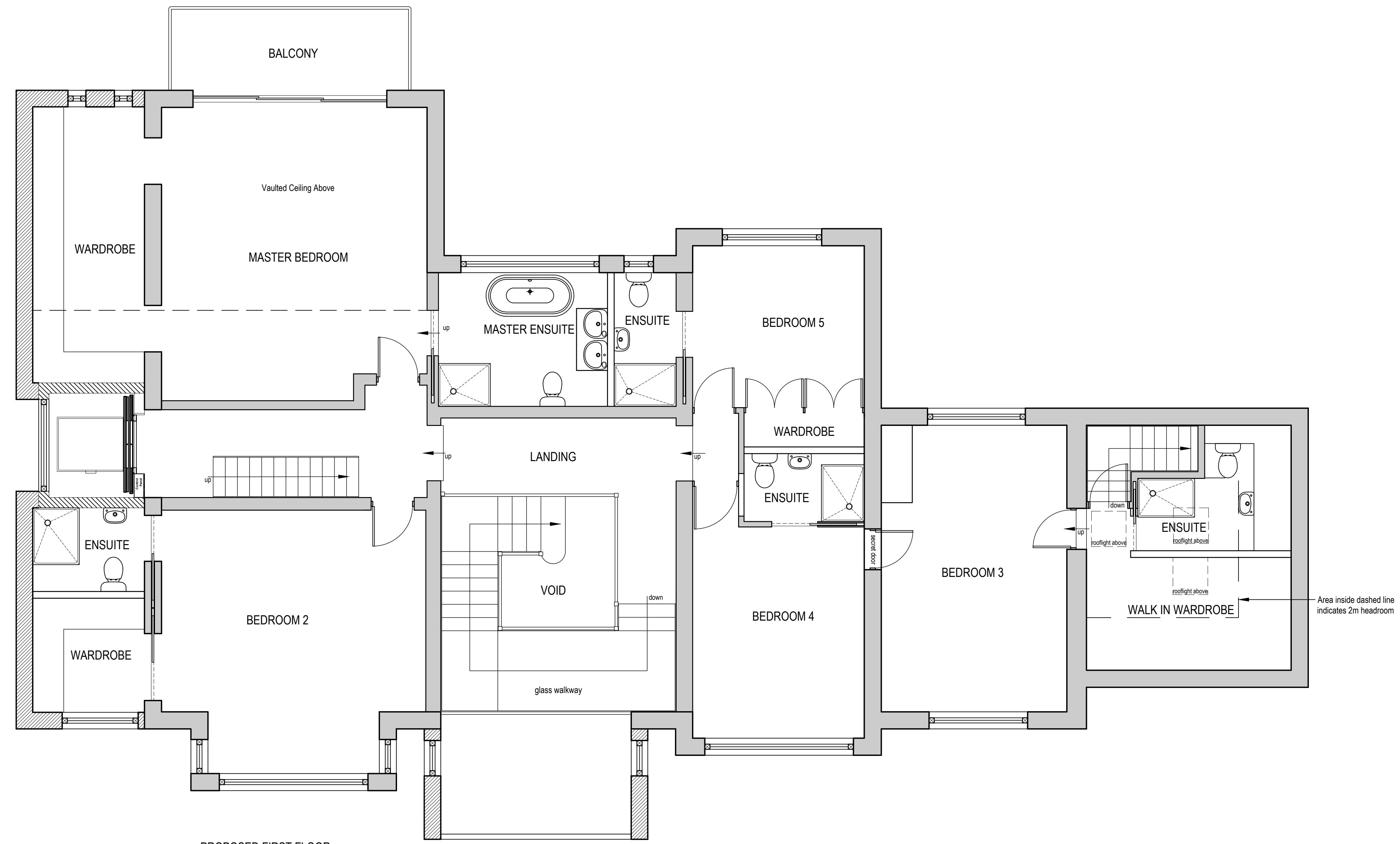
PROPOSED FIRST FLOOR PLAN (scale 1:50)
