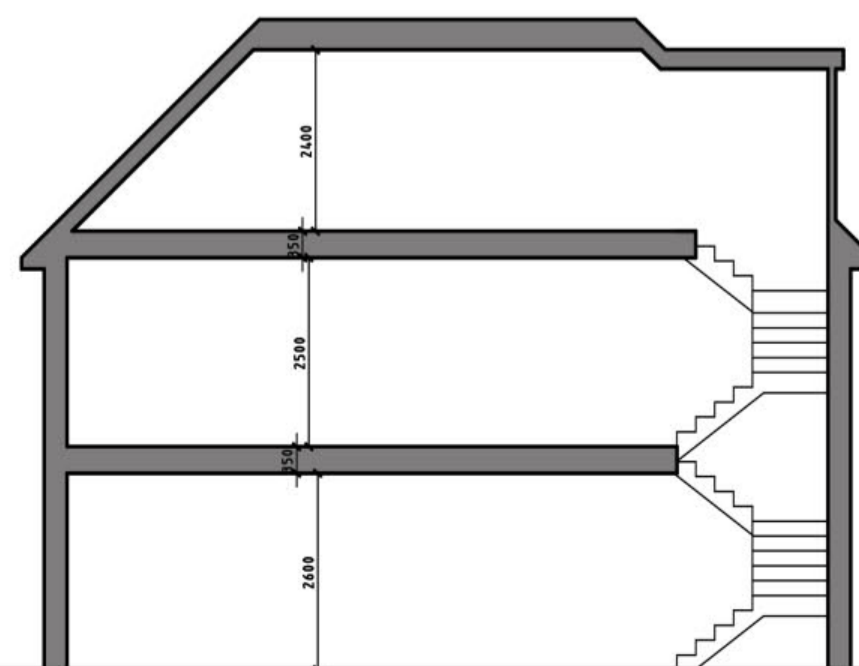
SECTION
