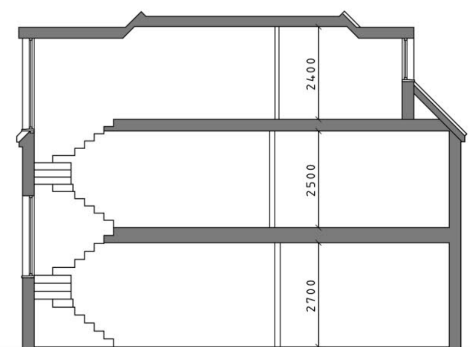
SHORT SECTION
