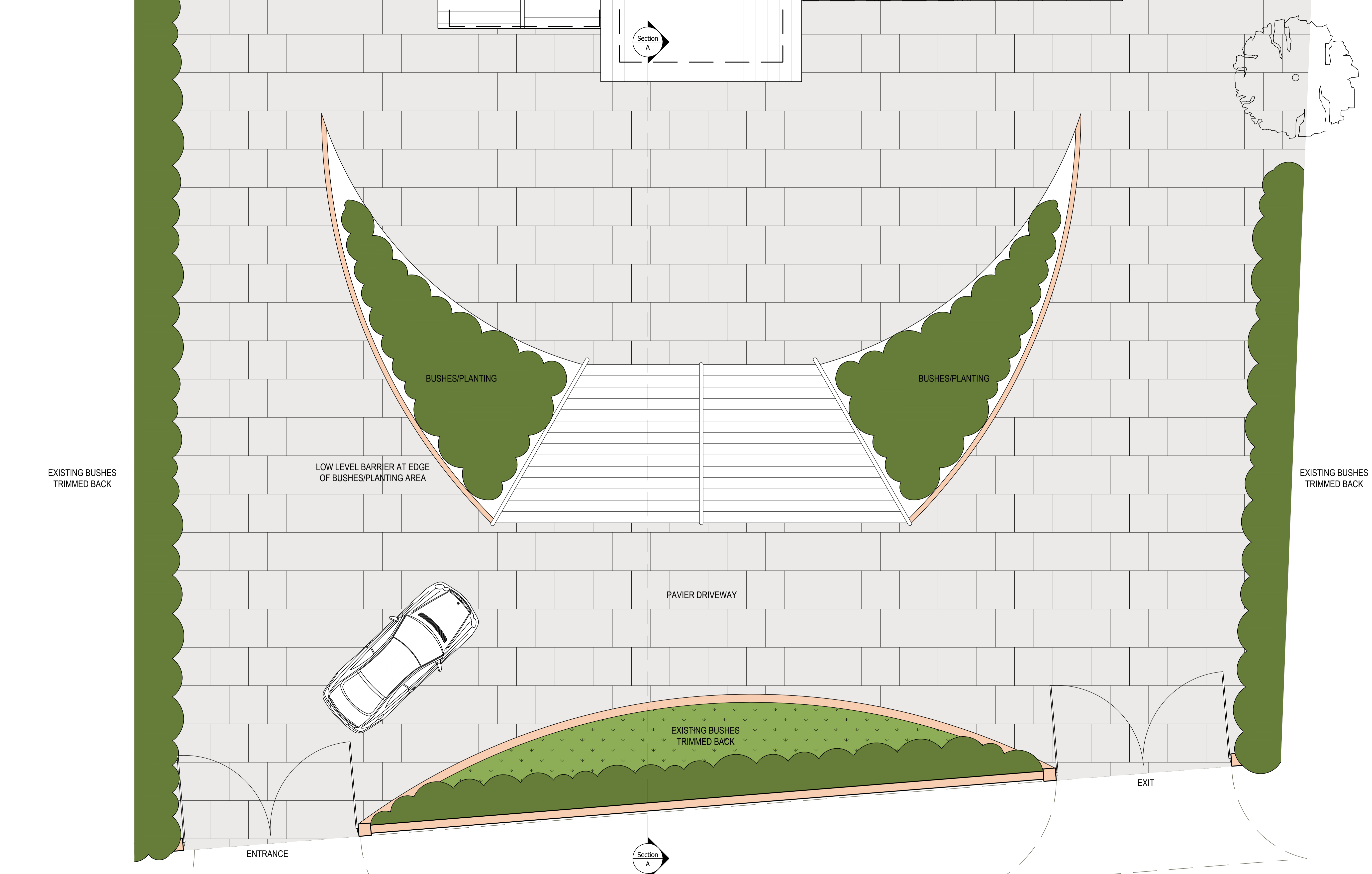
PROPOSED ACCESS PLAN (scale 1:50)
