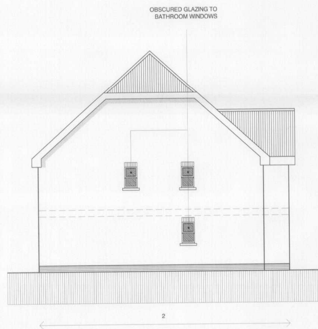
PLOT 2 - SIDE ELEVATION
