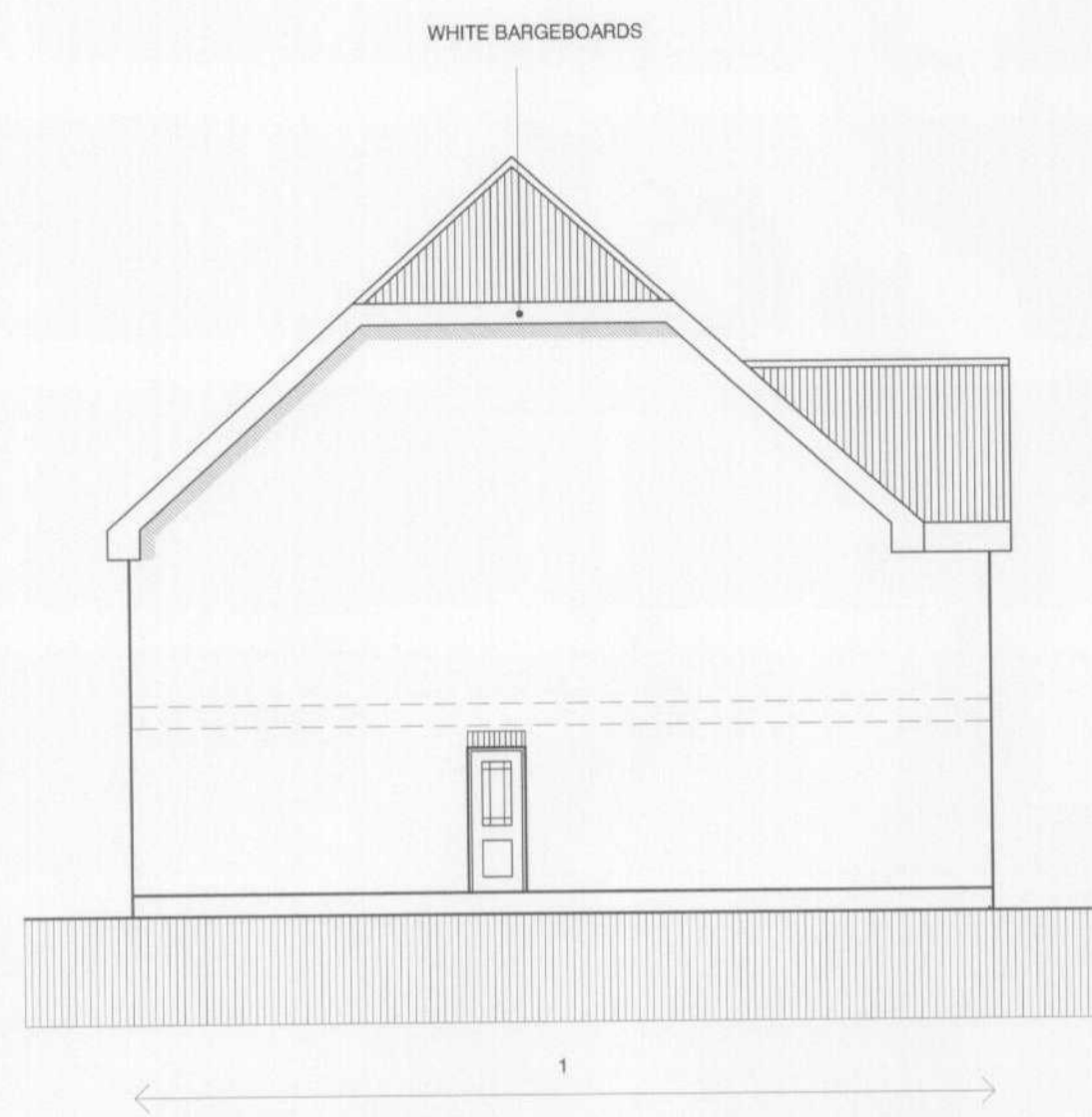
PLOT 1 - SIDE ELEVATION
