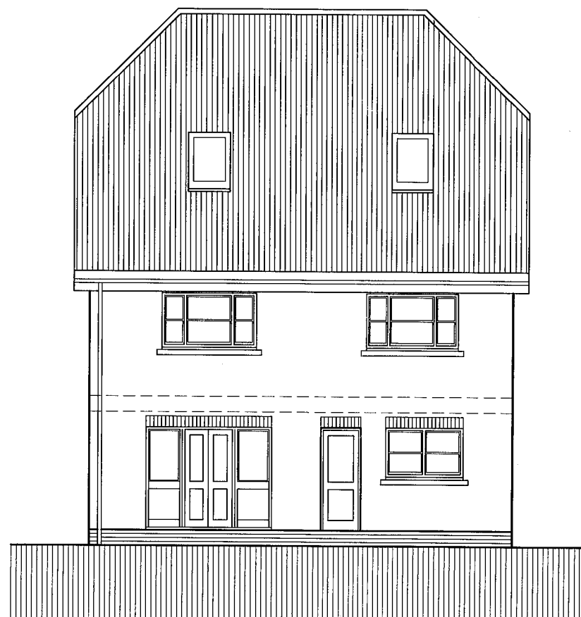
REAR ELEVATION
