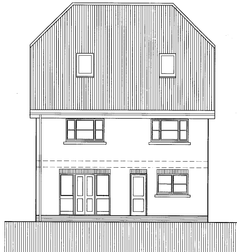
REAR ELEVATION
