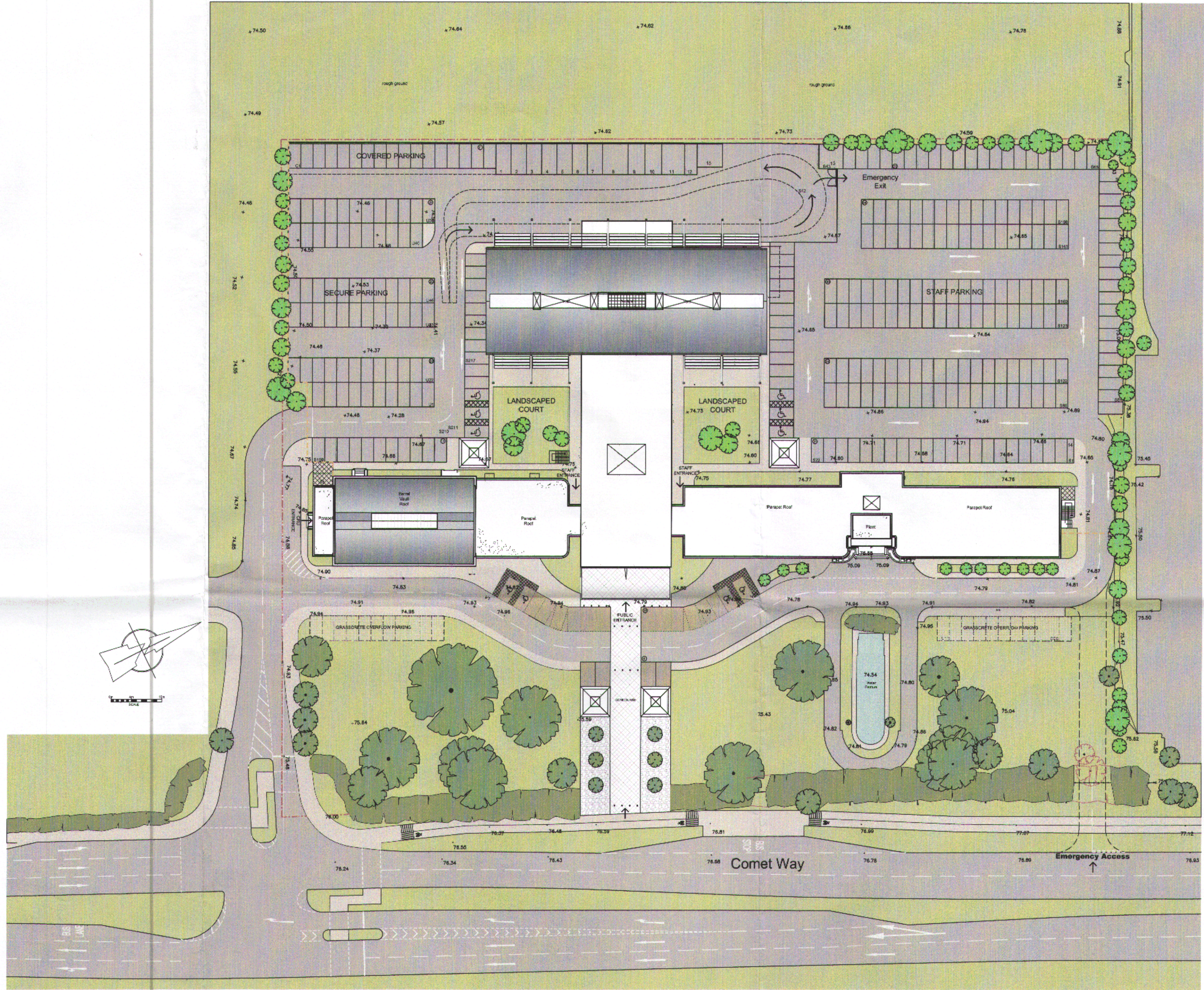
PROPOSED SITE PLAN
