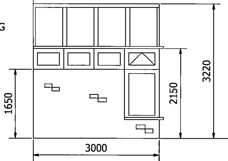
LEFT ELEVATION
