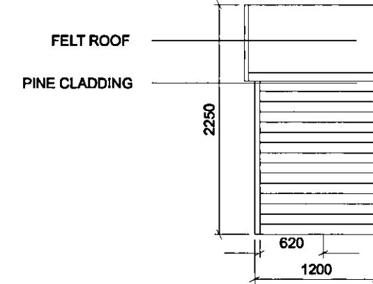
WEST ELEVATION
