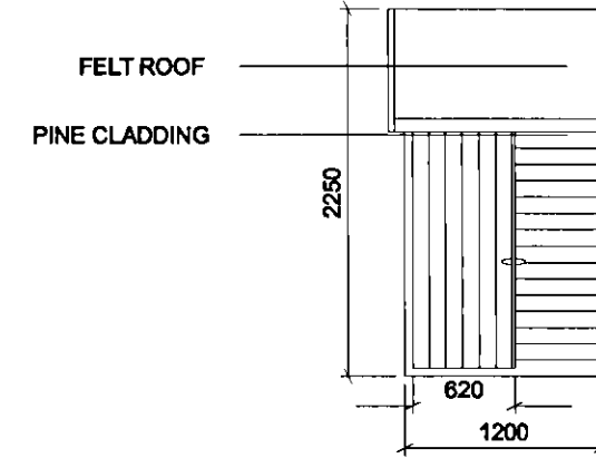
EAST ELEVATION
