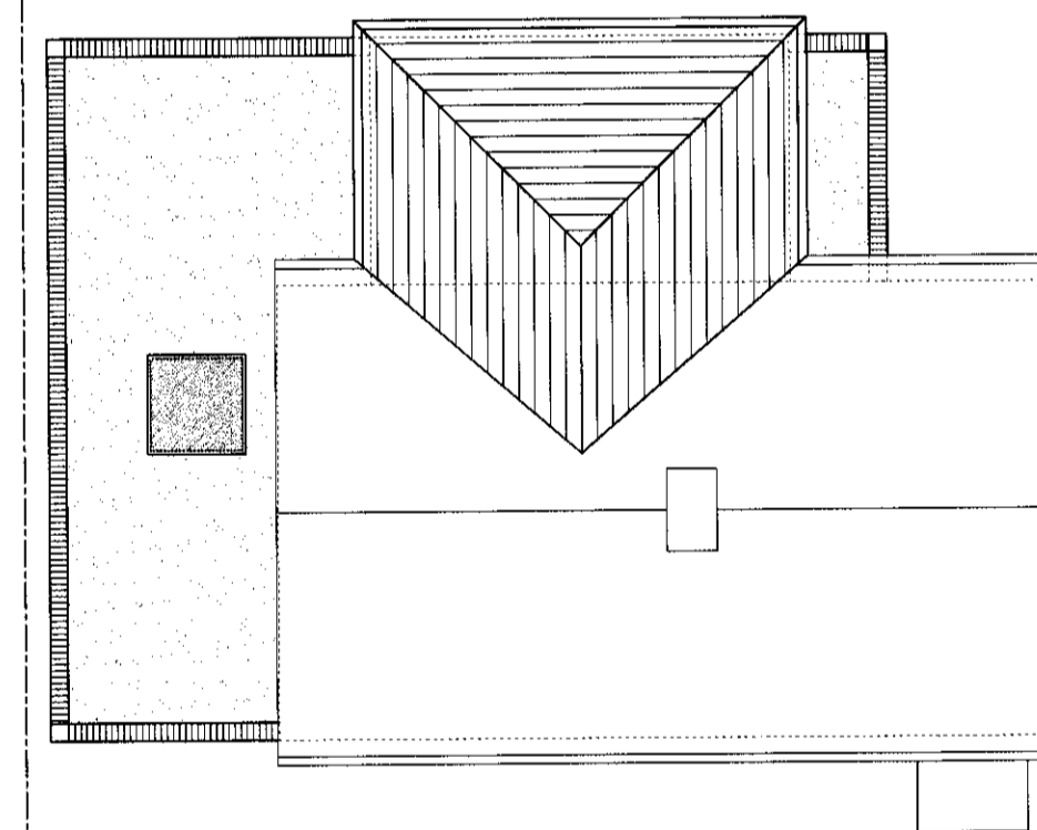
ROOF PLAN
