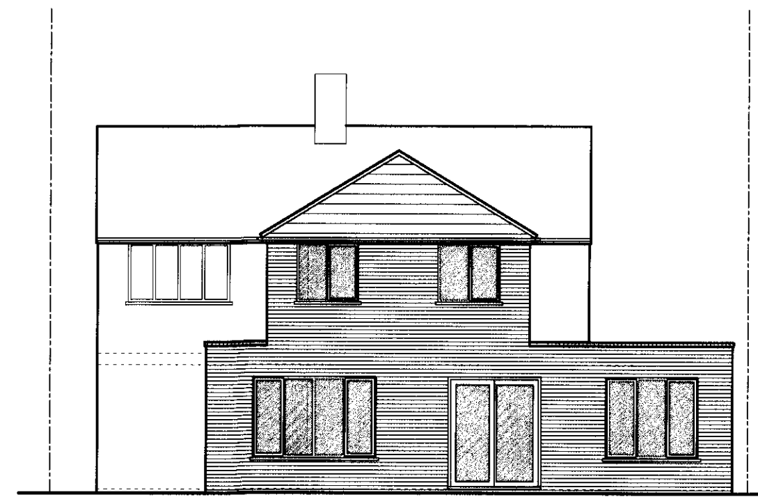
REAR ELEVATION
