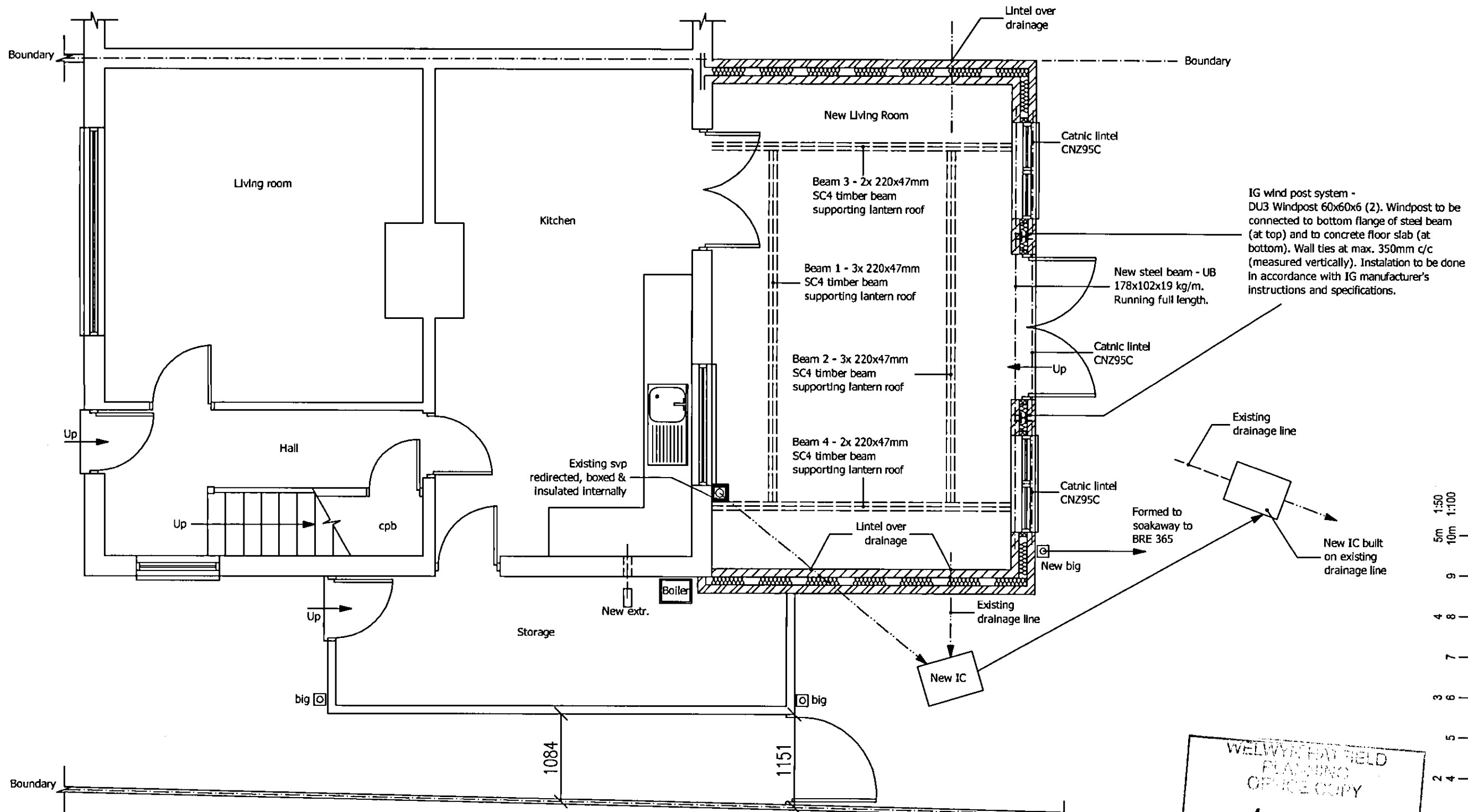
PROPOSED GROUND FLOOR PLAN scale 1:50
