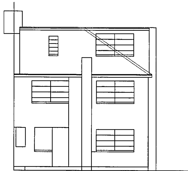
Rear Elevation
