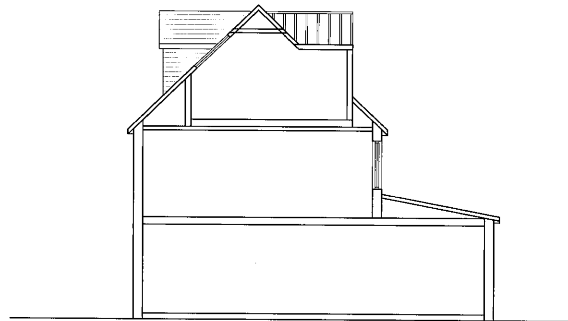
PROPOSED SECTION
