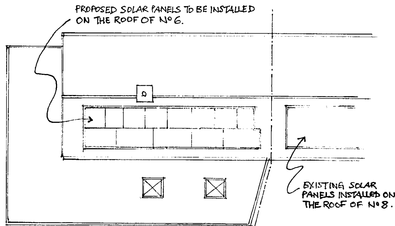
ROOF PLAN 1:100
