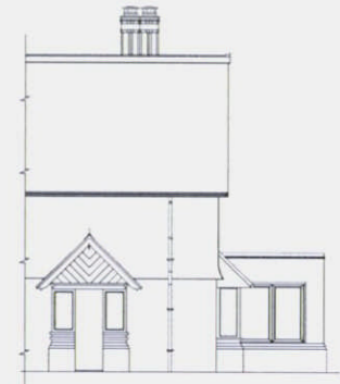
PROPOSED SIDE ELEVATION (A)
