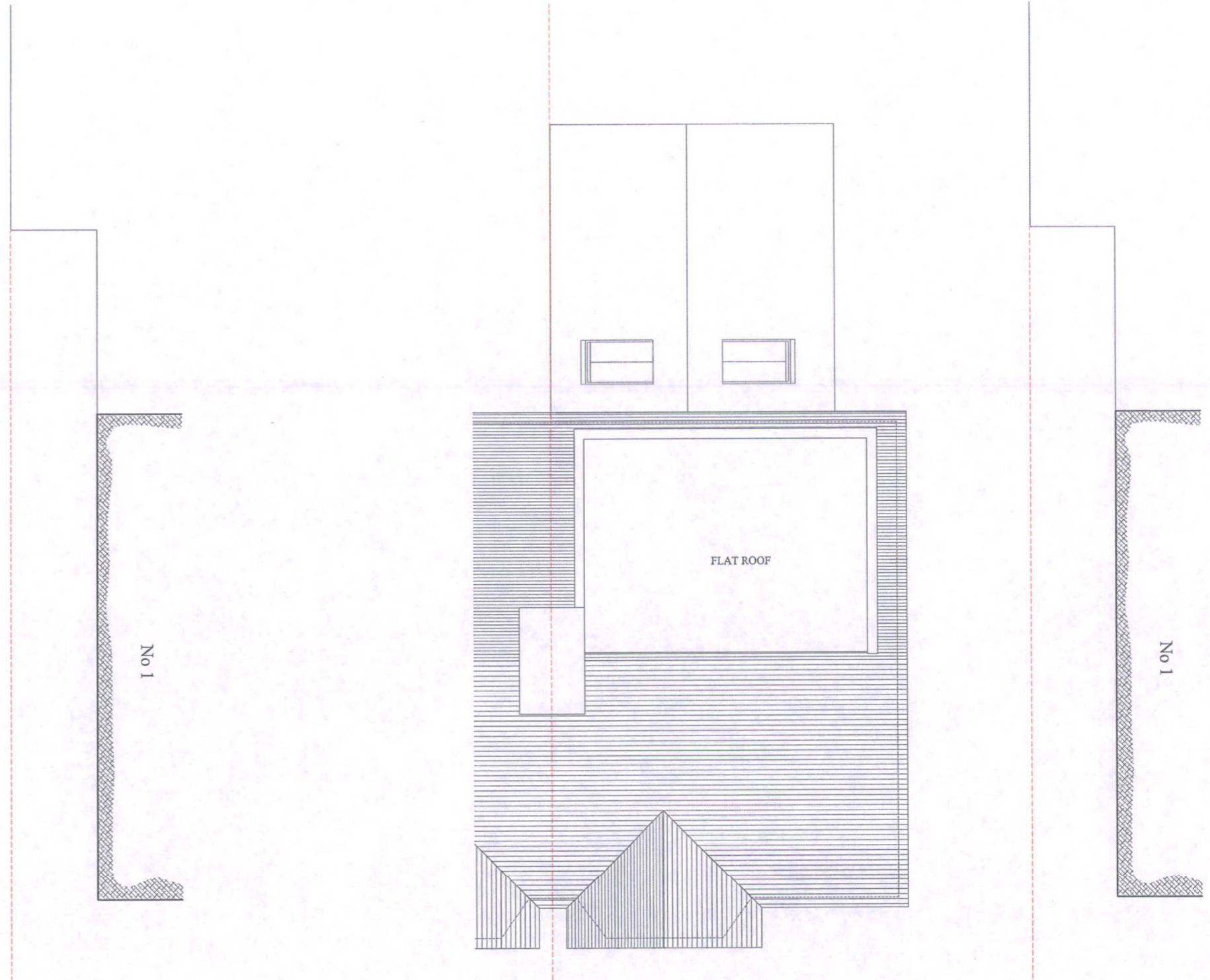
23 MANOR ROAD AL10 PROPOSED ROOF PLAN
