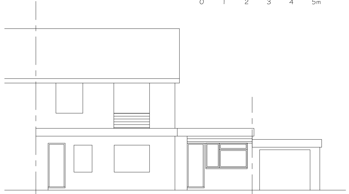
NORTH/E ELEVATION
