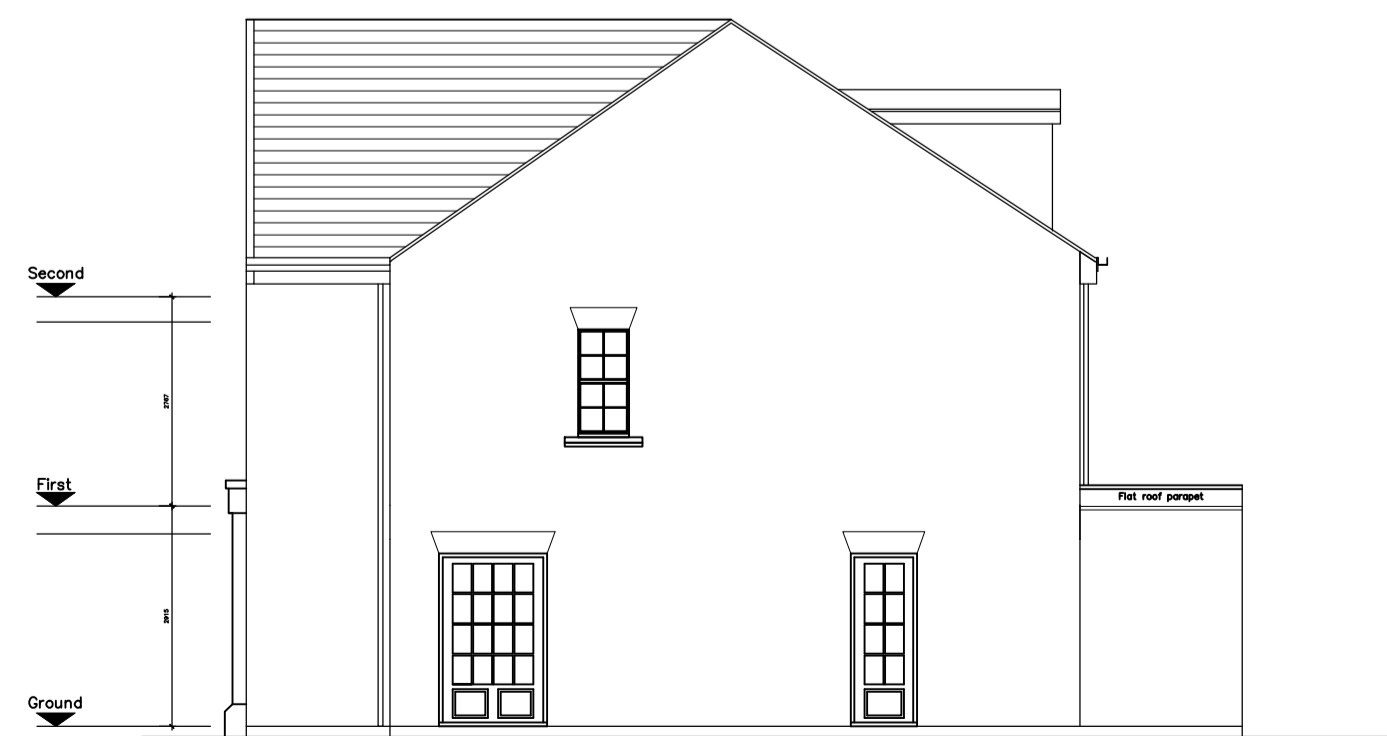
Side Elevation
