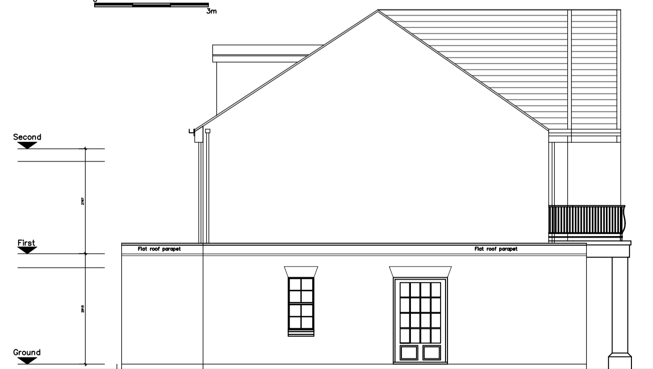
Side Elevation
