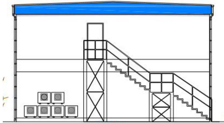
REAR ELEVATION
