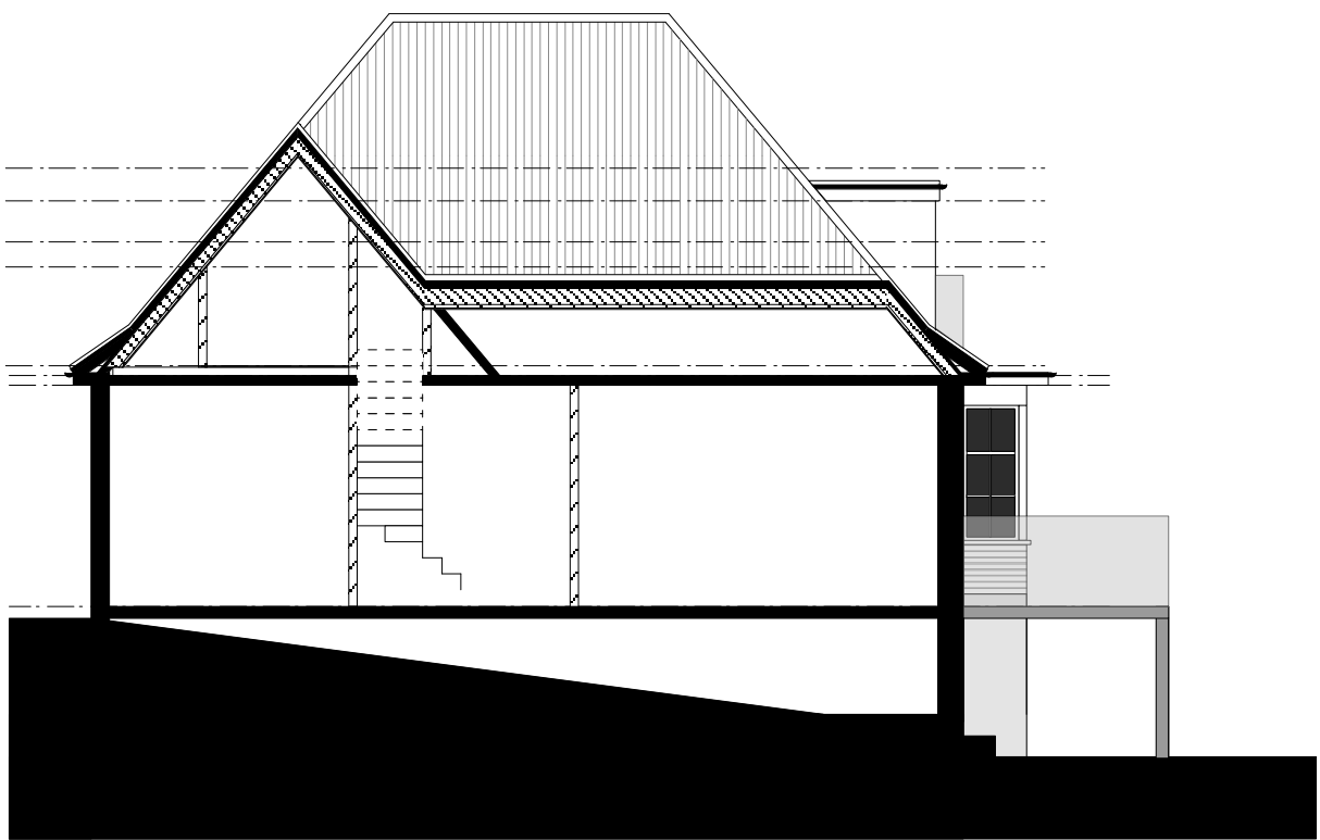
typical section
