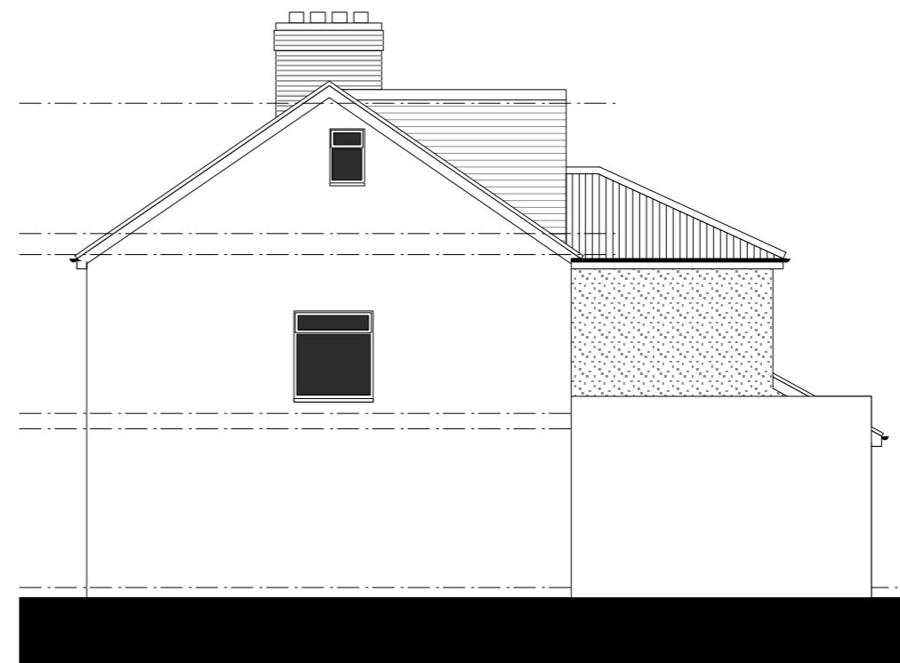
side elevation
