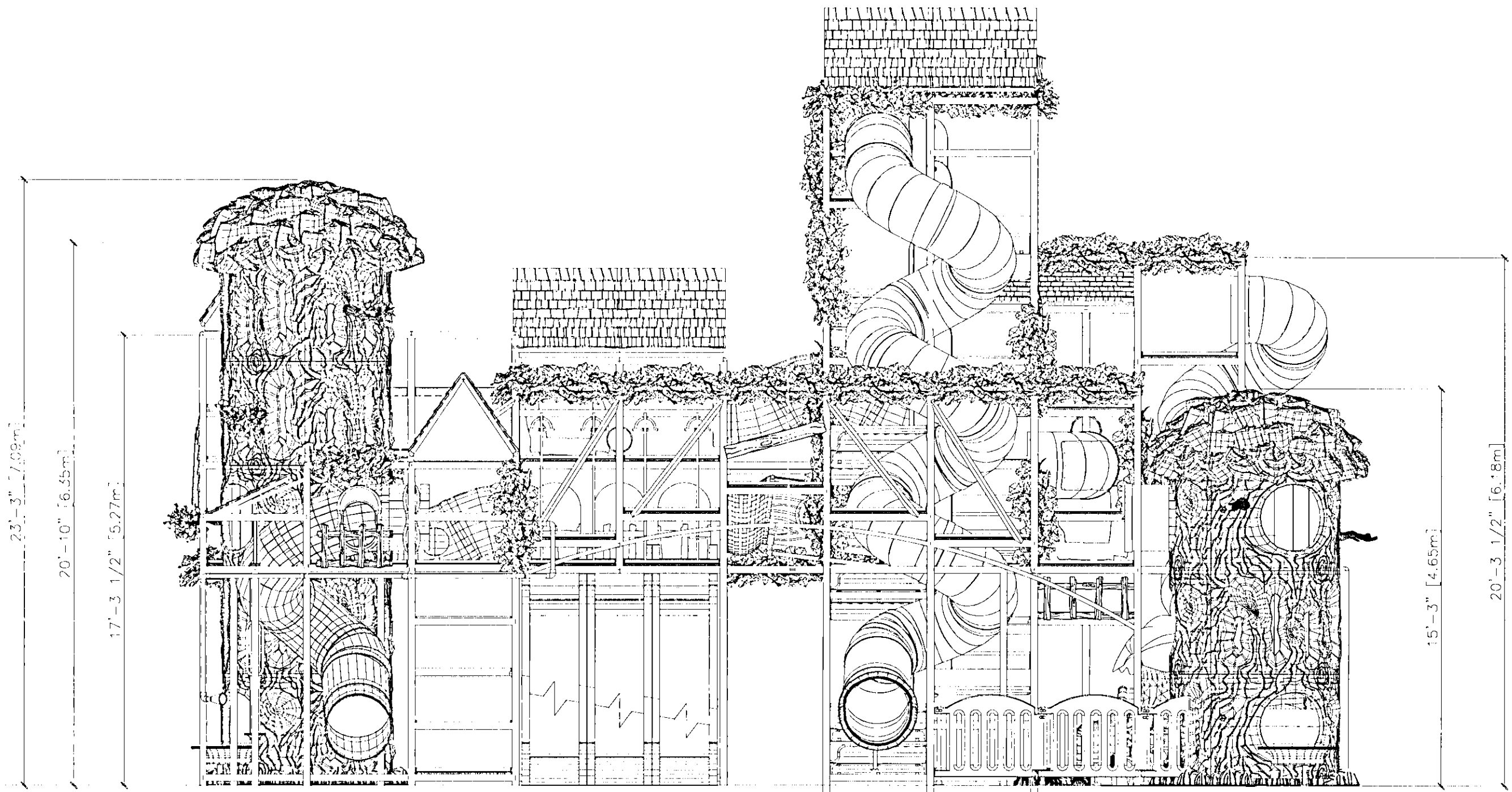
NORTH ELEVATION
