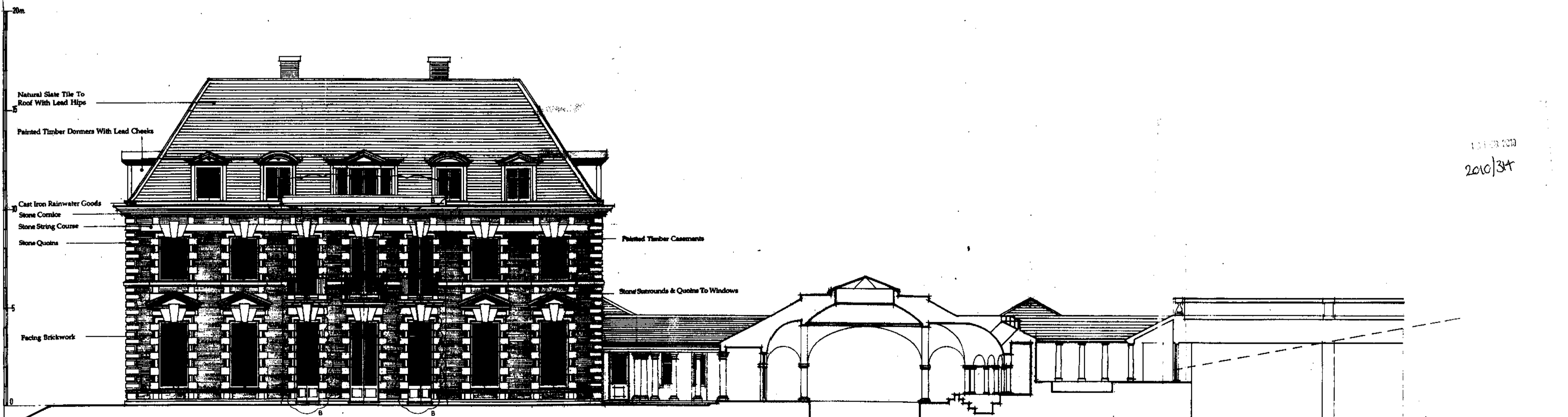
SOUTH EAST ELEVATION
