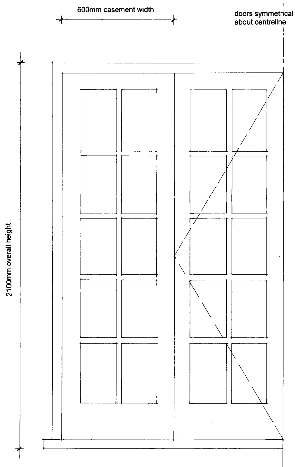
FRENCH DOORS ELEVATION 1:1
