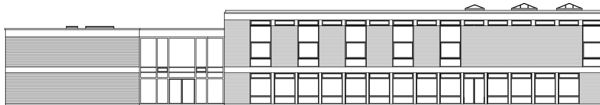
Existing East Elevation
