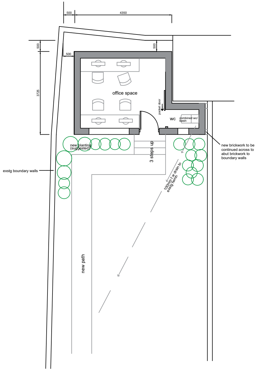
proposed floor plan scale 1:100 (amnd to show side & rear walls, min. 500mm from boundary walls)
