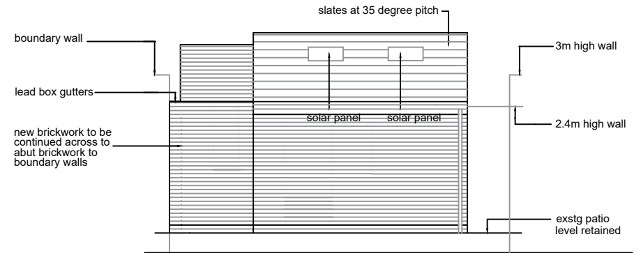
proposed rear elevation scale 1:100
