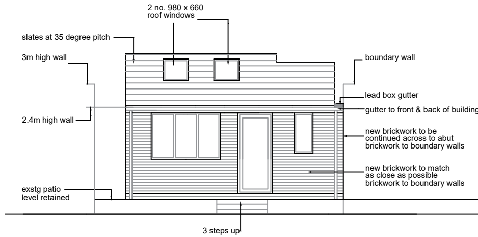
proposed front elevation (amnd to show side & rear walls, min. 500mm from boundary walls)
