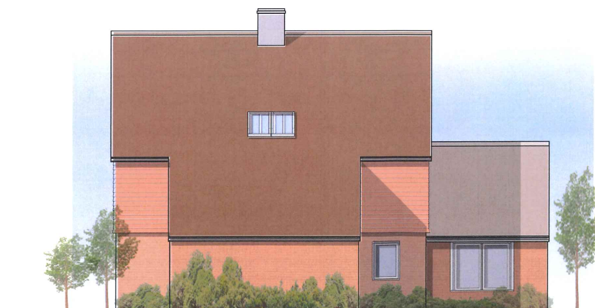
WEST ELEVATION
