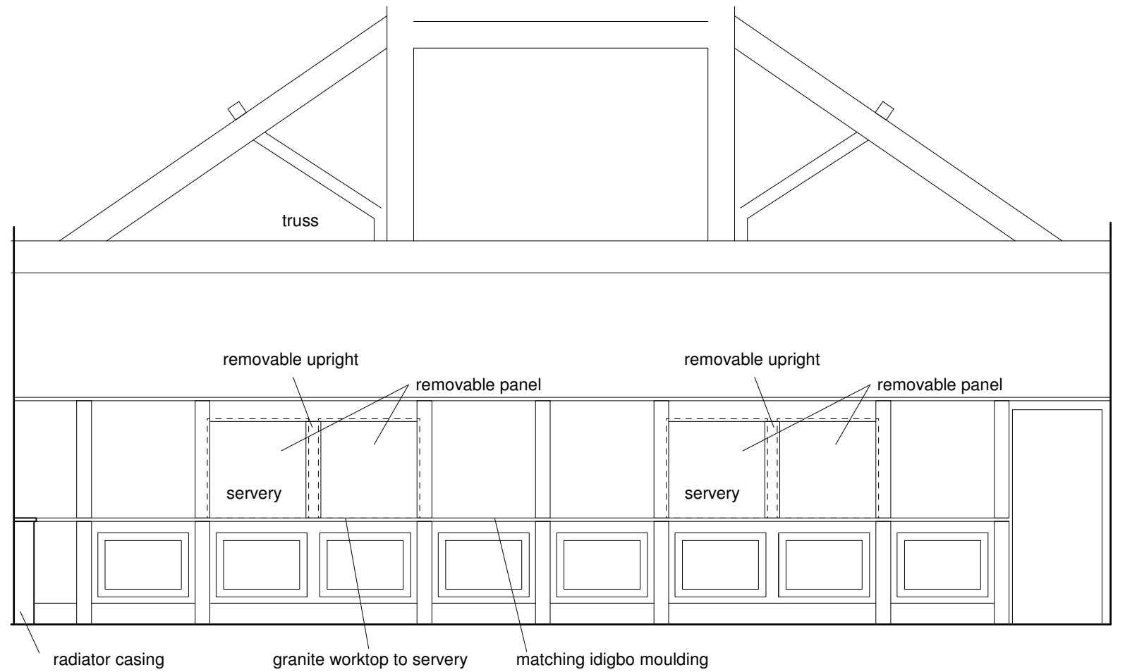
SERVERY ELEVATION
