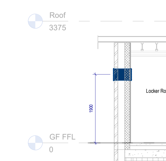
9 Section_Locker Room 1:50
