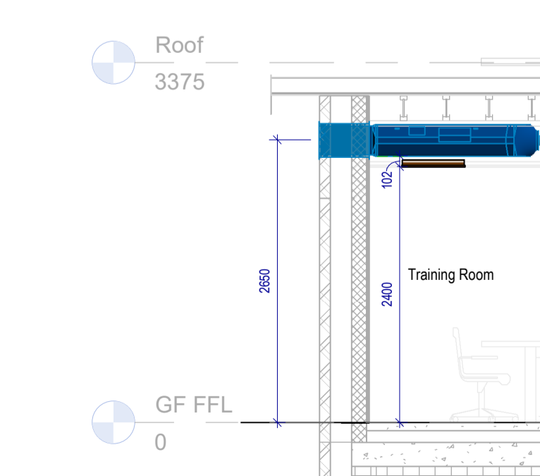
10 Section_Training Room 1:50
