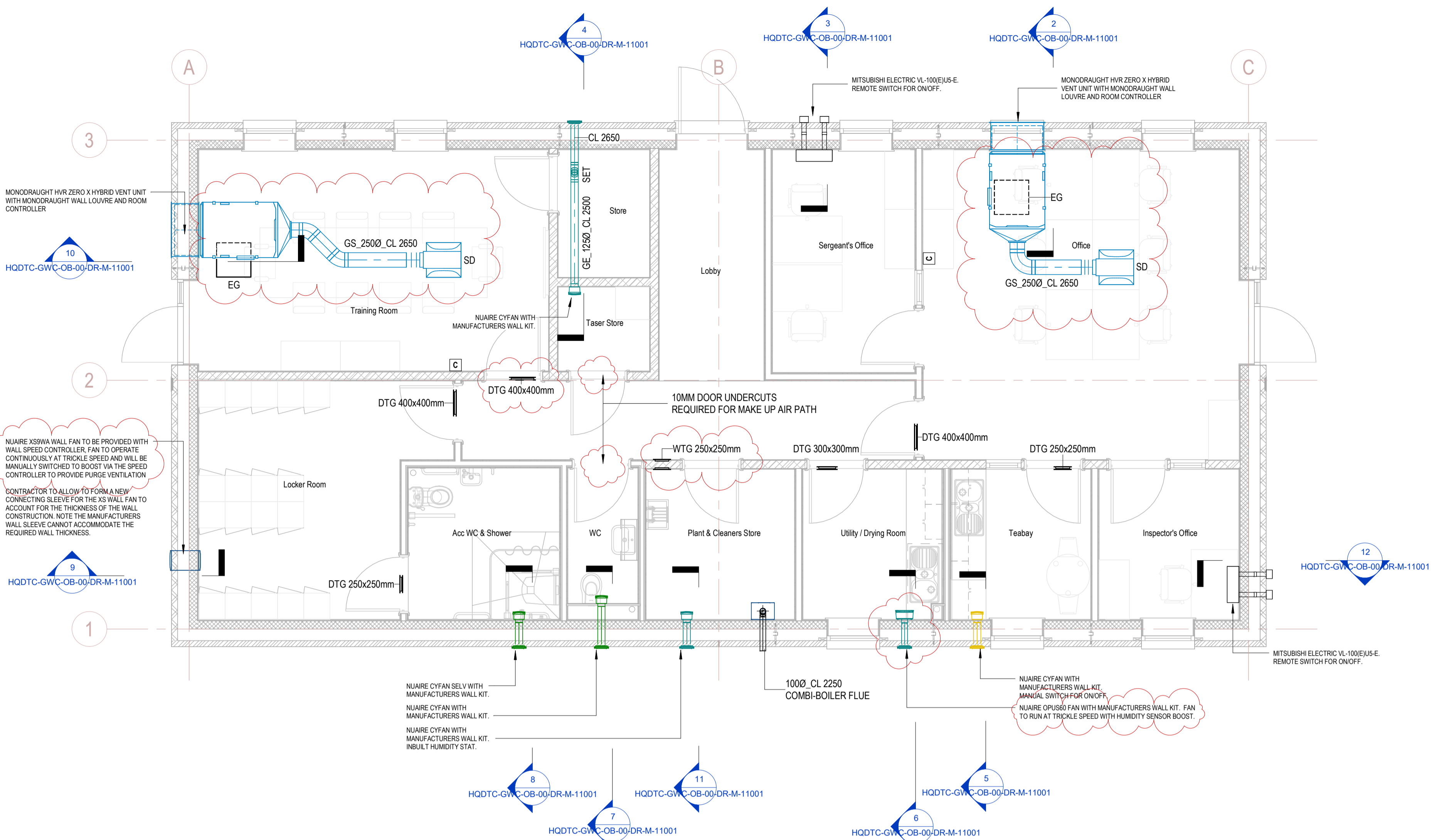
1 OB_00_Ventilation 1:50
