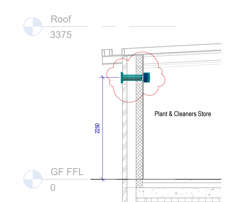
11 Section_Plant 1:50
