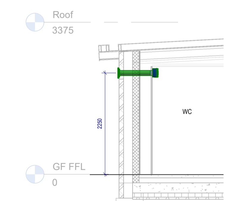
7 Section_WC 1:50
