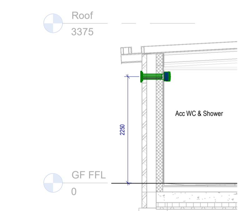
8 Section_AccWC/Shower 1:50
