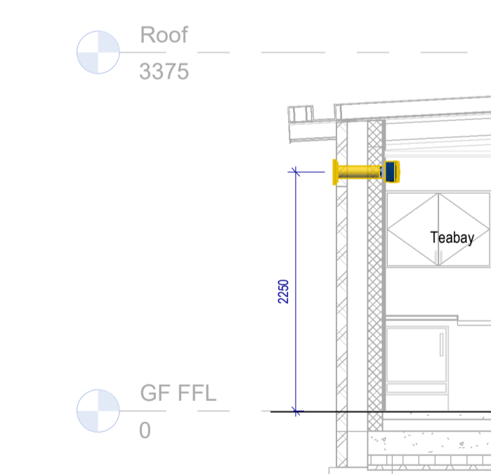
5 Section_TeaBay 1:50
