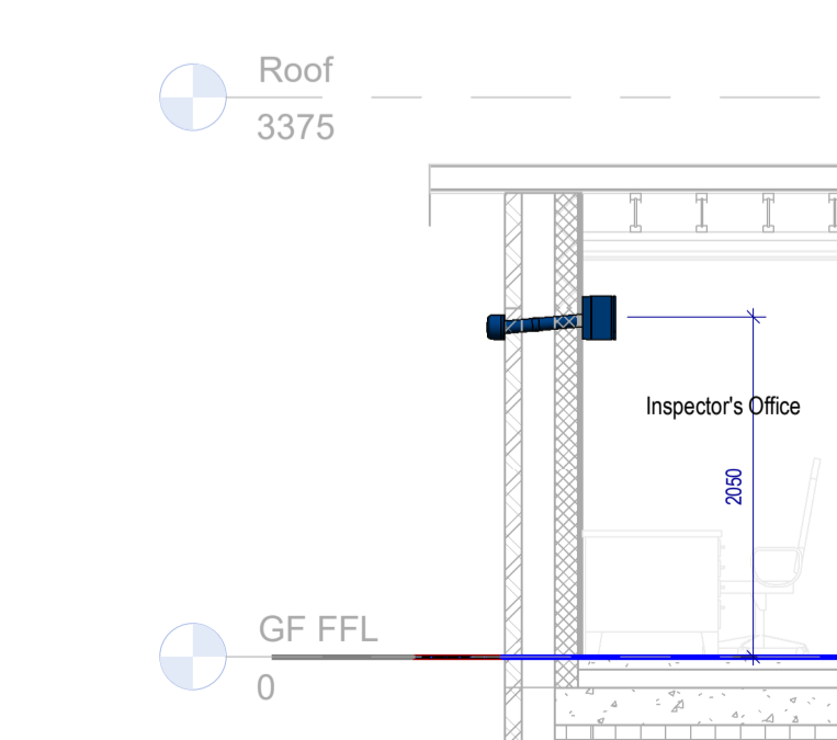
12 Section_Inspector's Office 1:50
