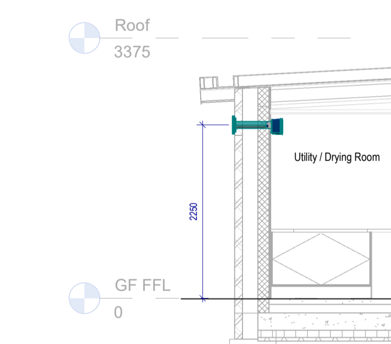
6 Section_Utility/Drying Room 1:50
