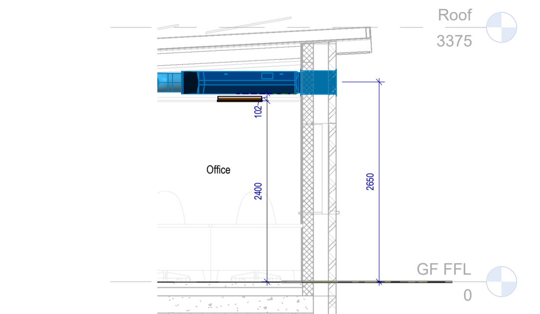
2 Section_Office 1:50
