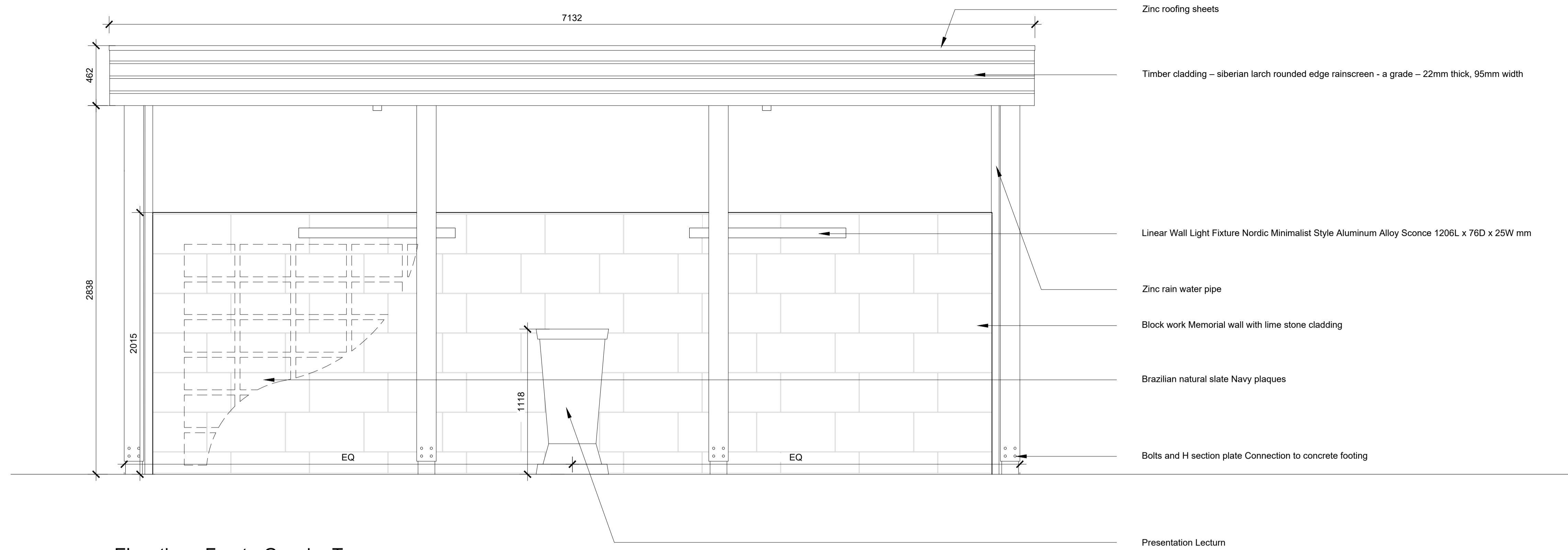
Elevation - Front - Gazebo Two
