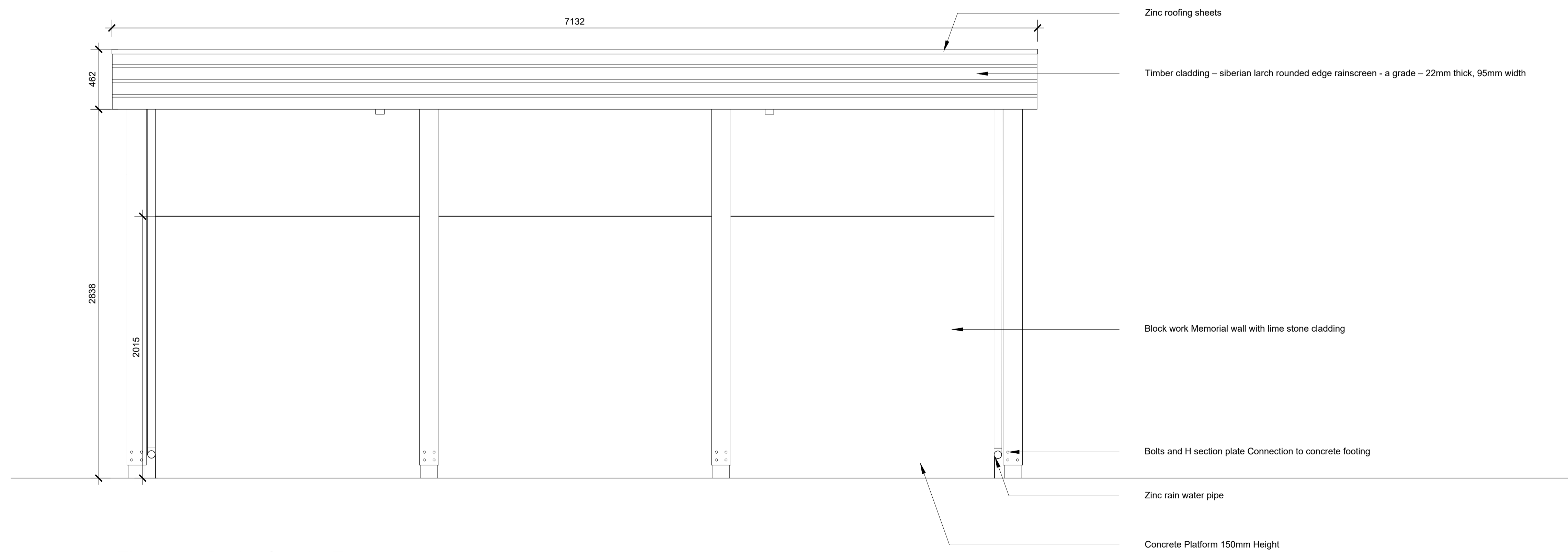
Elevation - Back - Gazebo Two
