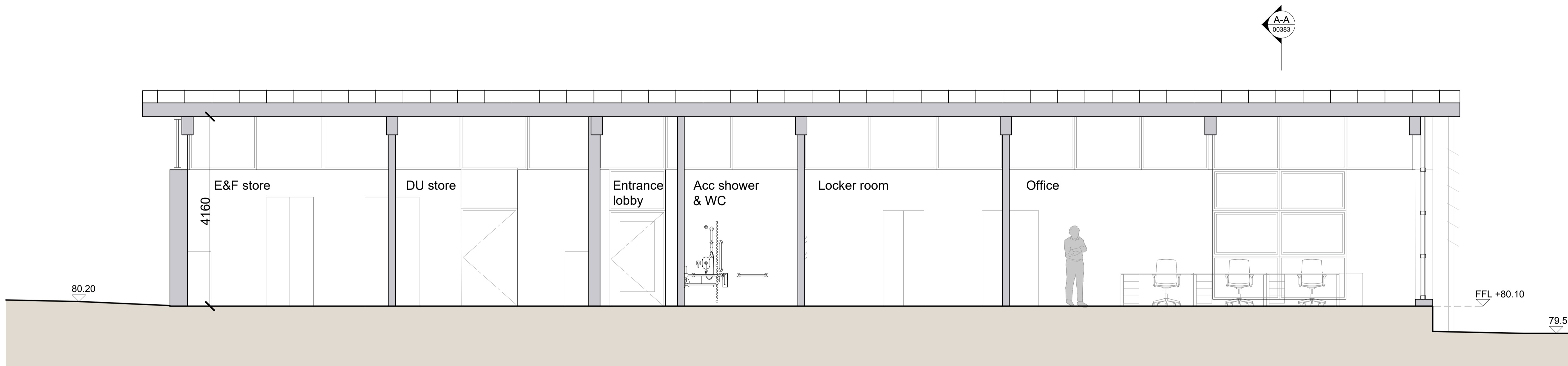
Section B-B
