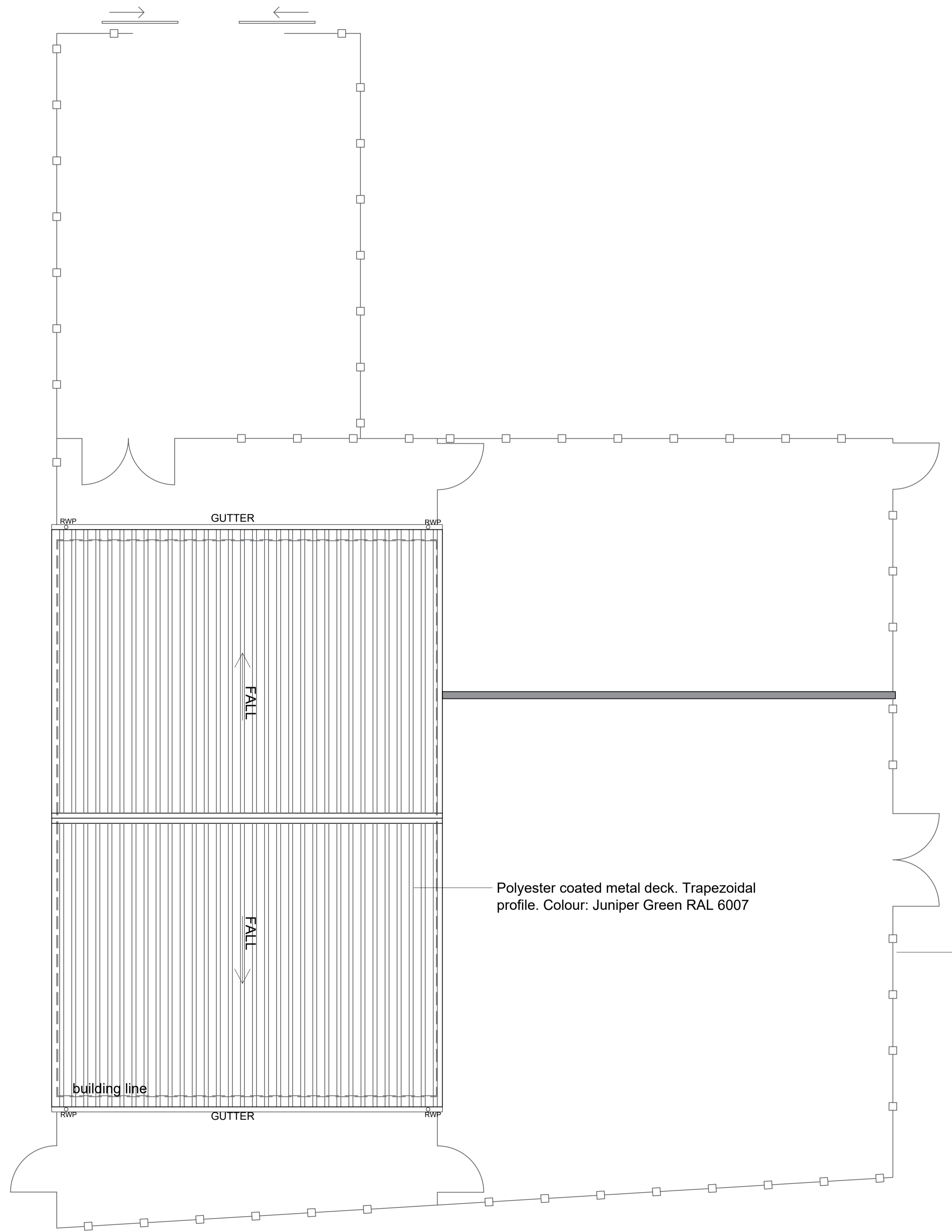
Roof Plan
