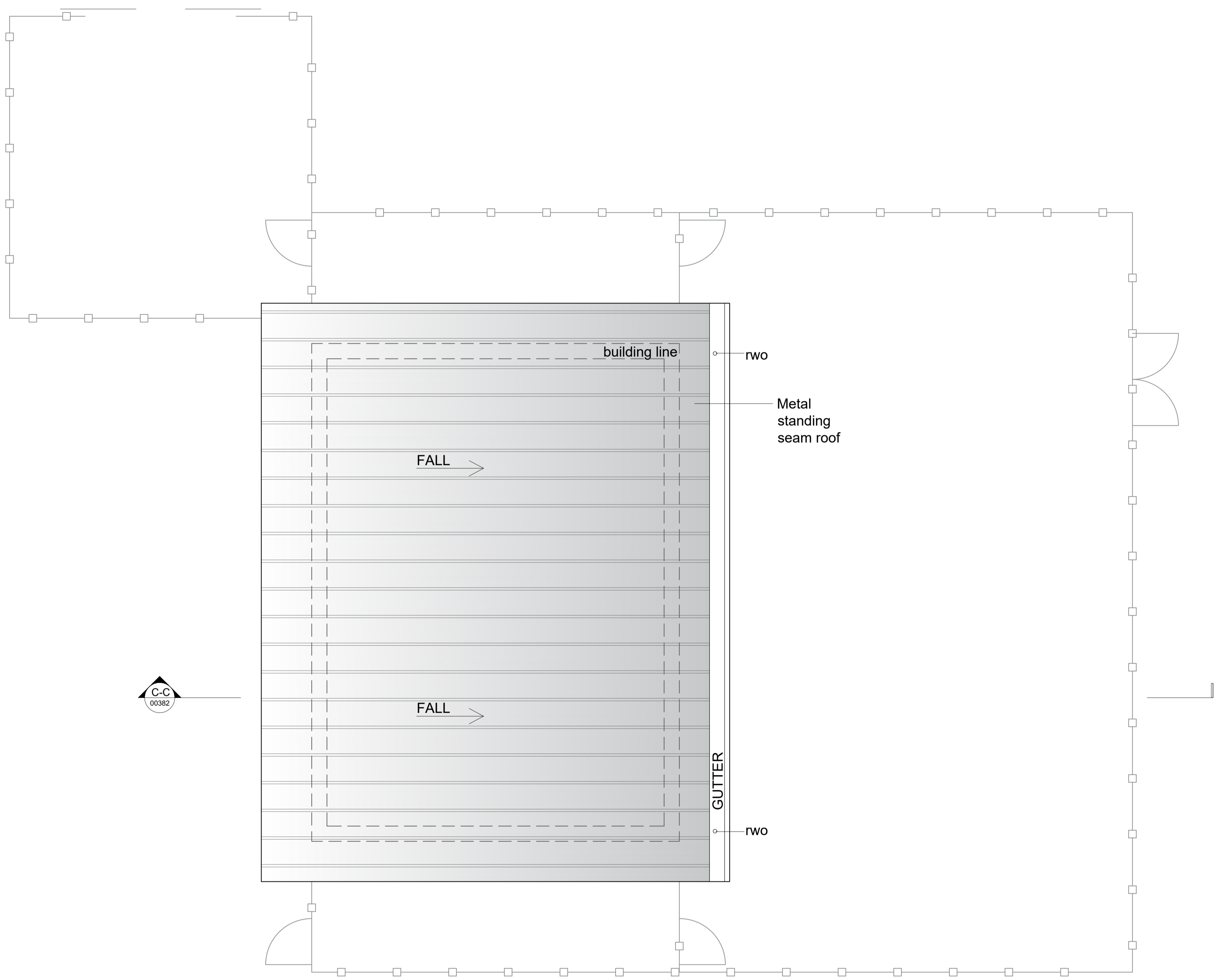
Roof Plan
