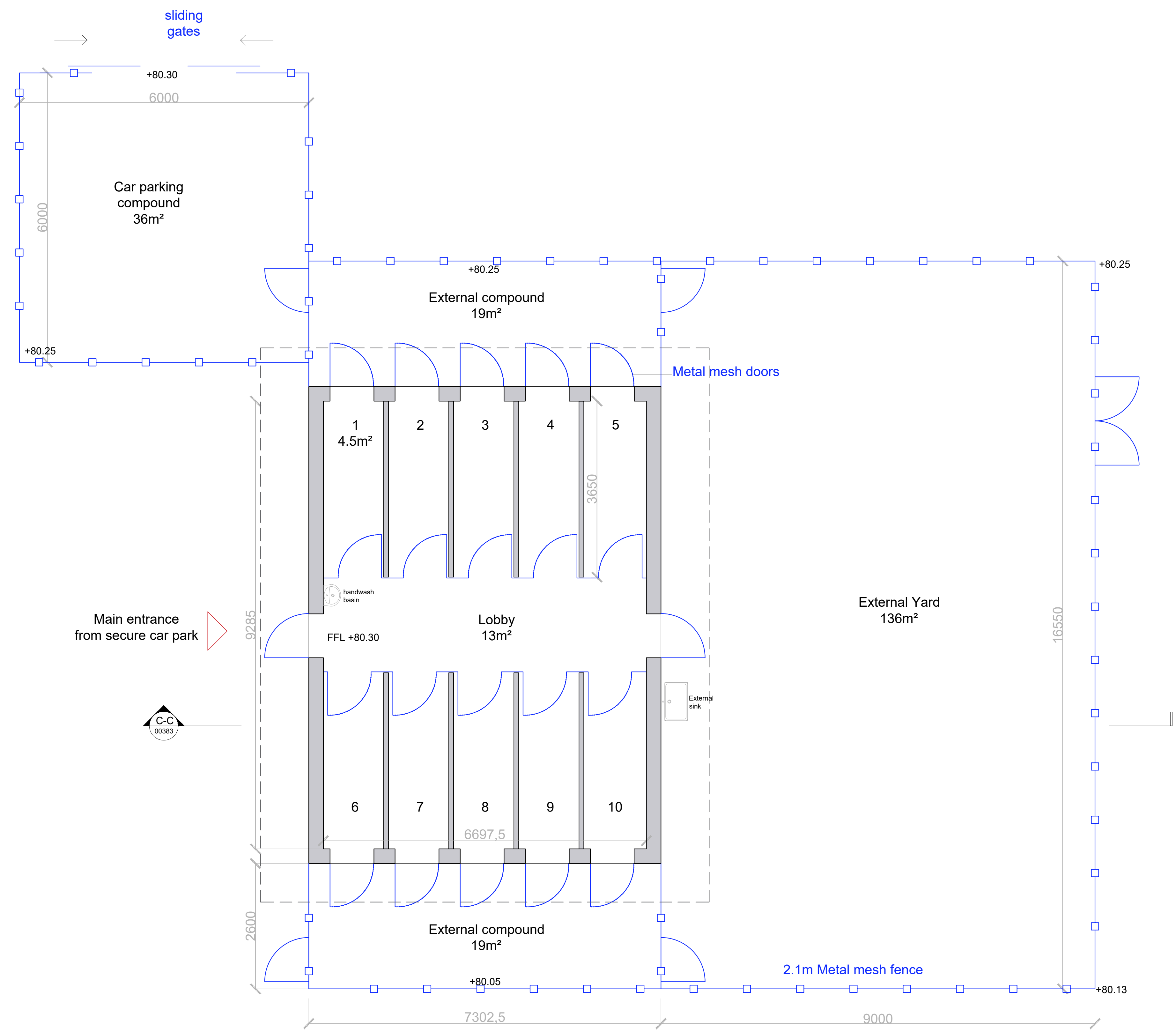
Ground Floor Plan GIFA - 62m 2
