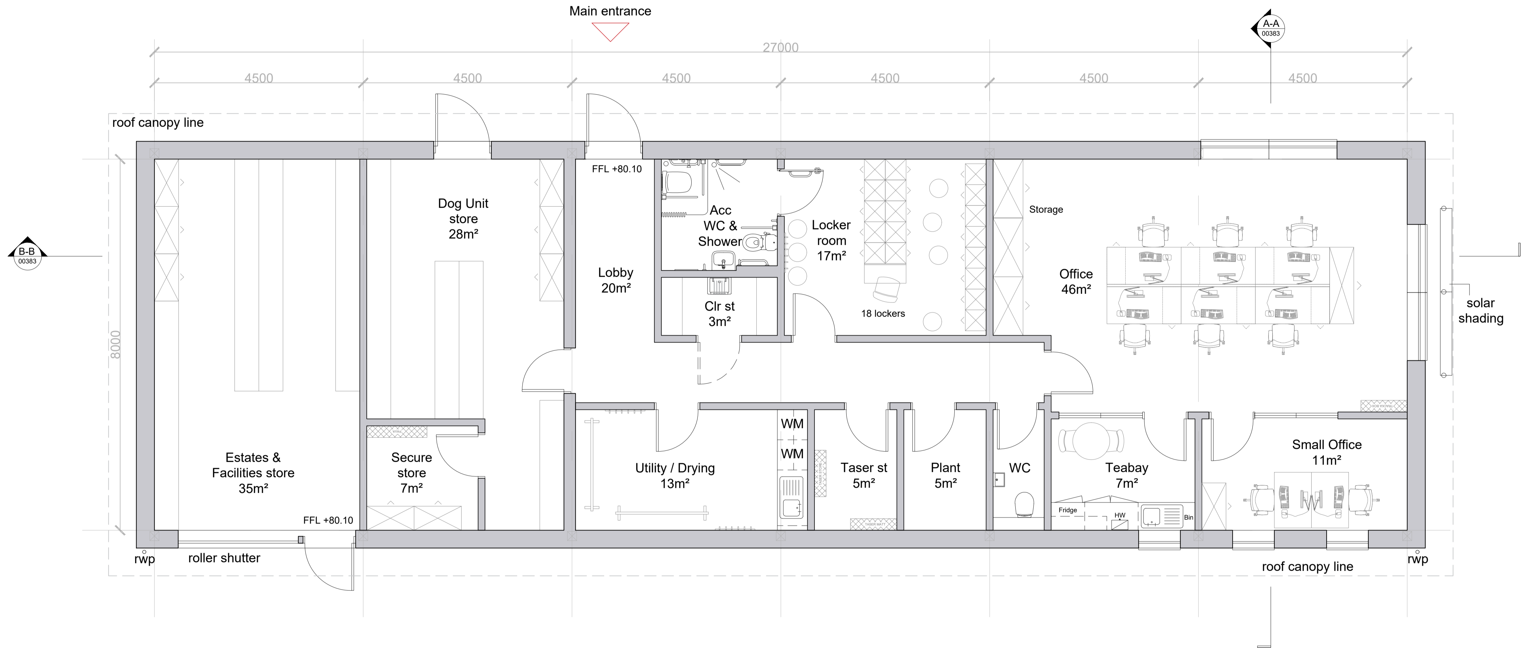
Ground Floor Plan GIFA - 216m 2
