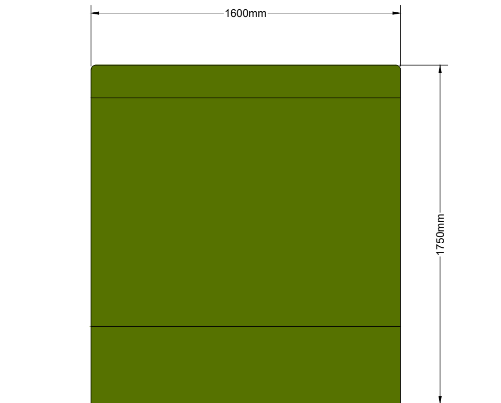
BACK ELEVATION
