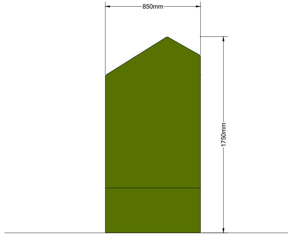
SIDE ELEVATION
